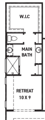
OPT. RETREAT@ MAIN BEDROOM +106 SQ. FT.
