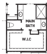
MAIN BATH W/ SPLIT VANITY OPT.
