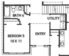
OPT. BEDROOM 5/ BATH 4 @ LIVING
