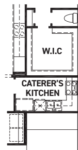
OPT. CATERER'S KITCHEN +73 SQ. FT.
