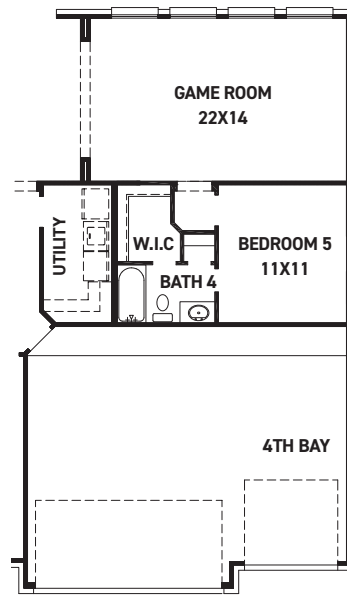
OPT. 4TH BAY, GAME ROOM & BEDROOM 5 *NOT AVAIL. W/ 2ND FLOOR OPTIONS +272 SQ. FT.
