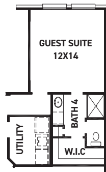
OPT. GUEST SUITE +127 SQ. FT.
