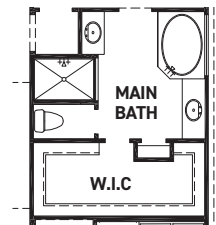
OPT. ENLARGED MAIN SHOWER W/ TUB
