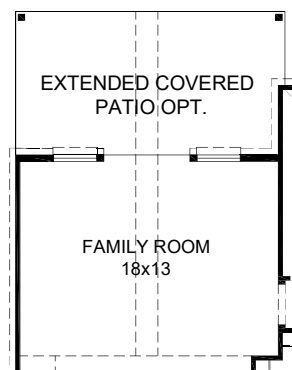
POINTED VAULT OPT. W/ EXTENDED COVERED PATIO
