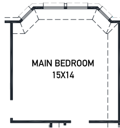
OPT. MAIN BEDROOM BAY
