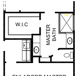
W.I.C. MASTER BATH ENLARGED MASTER SHOWER OPTION
