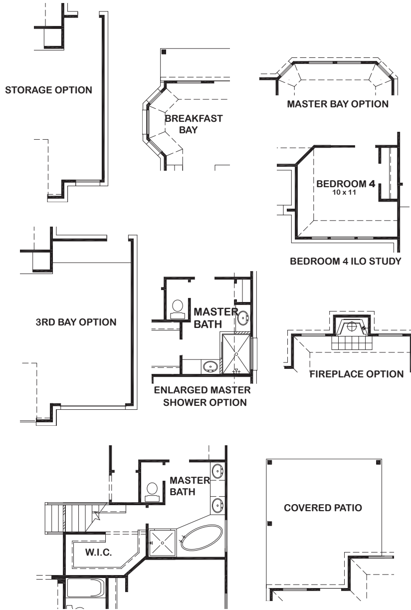
FIRST FLOOR W/ SECOND FLOOR OPT.
