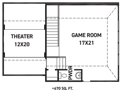
SECOND FLOOR OPTIONS
