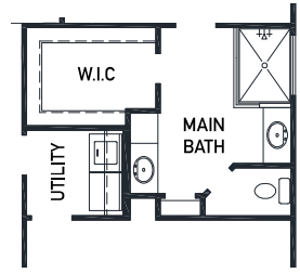
OPT. ENLARGED MAIN SHOWER
