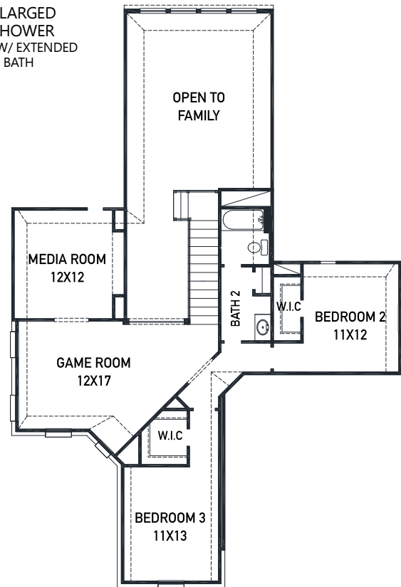
SECOND FLOOR PLAN REV 8/20 (5508)
