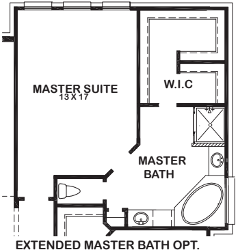
EXTENDED MASTER BATH OPT.
