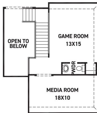
OPT. SECOND FLOOR GAME ROOM & MEDIA
