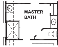
ENLARGED MASTER SHOWER OPTION NOT AVAILABLE W/EXTENDED MASTER BATH OPTION
